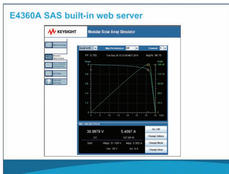
Figure 4: Keysight E4360A built-in web server
